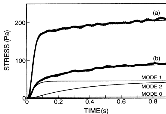
FIG. 2. Typical stress responses to a stepwise electric field at shear rates of (a) 4.1 \text{ s}^{-1} and (b) 0.54 \text{ s}^{-1} . Amplitude of the electric field was 2 kV/mm. Viscosity of the continuous phase was 0.02 \text{ Pa s} , \epsilon_c was 2.70, and \beta was 0.90. Fitted curves and the components (mode 0, mode 1, and mode 2) of the fitted curve (b) are also shown in the figure.
